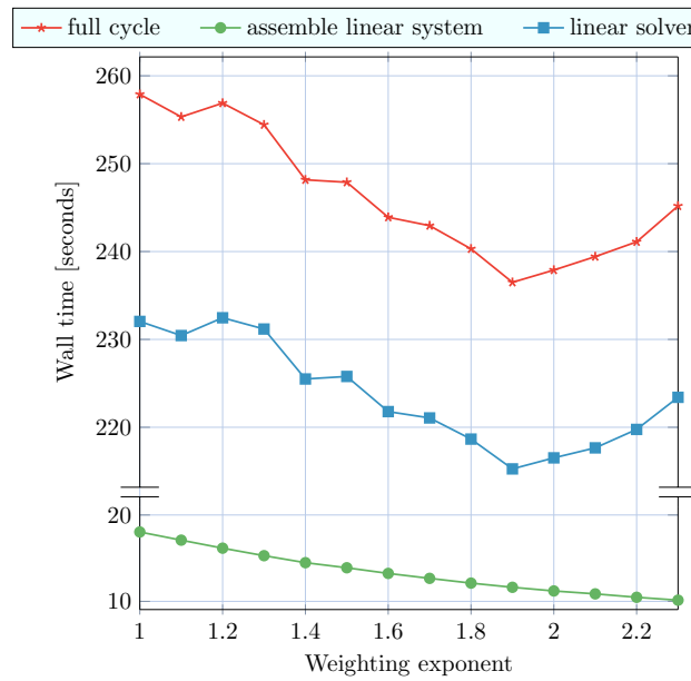
Figure 4.6: Wall times of a complete adaptation cycle and those parts relevant for load balancing. The problem has about 46 million DoFs and is solved on two nodes or 96 MPI processes. Weights proportional to n_{\text{dofs}}^c will be assigned to each cell with varying exponents c .
