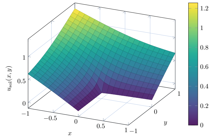
Figure 4.1: Solution of Eq. (4.3) for the manufactured Laplace problem on the L -shaped domain described by Eq. (4.7).
